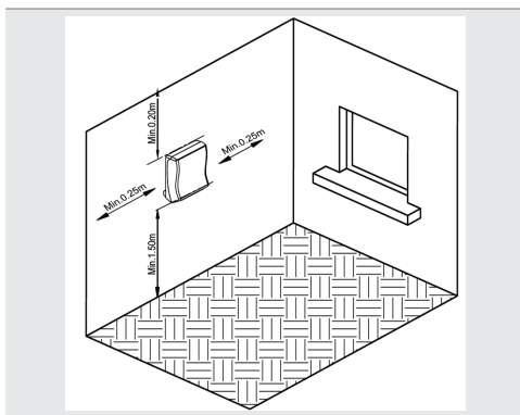
Fig.2: Assembly dimensions
